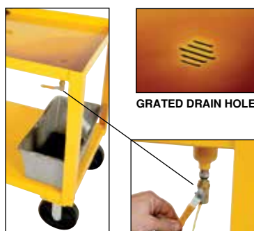
BALL VALVE
